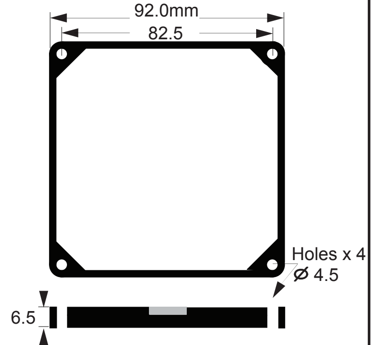
Guard "G" / G92PS
