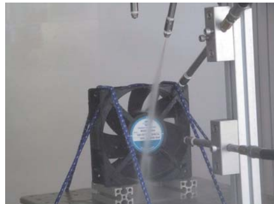
2-4 IPX9K Testing 60°
